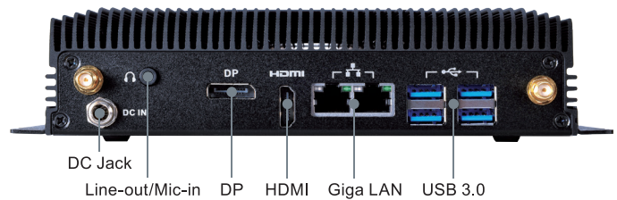
Rear I/O
